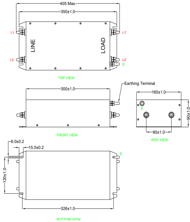
screw terminal
